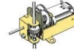
70110 4-SPEED CRANK AXLE GEARBOX
